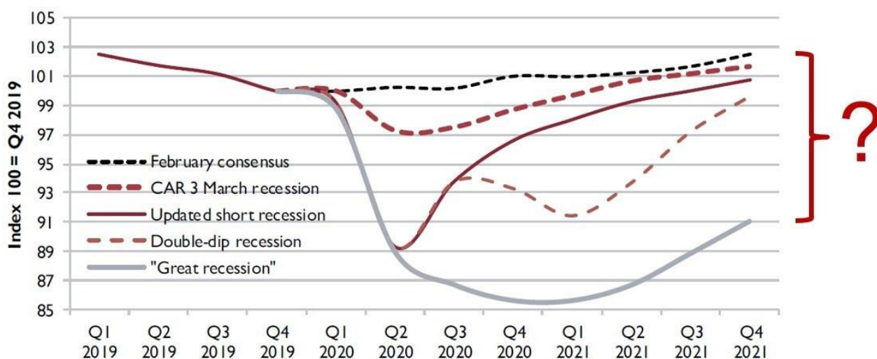
Schematic scenarios for Eurozone industrial production
